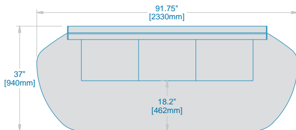
LINEAR C-TOP EDGE DETAIL FC-GCX-W3-B
