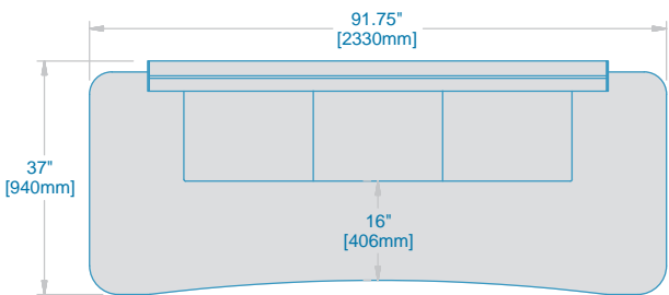
SCALLOPED C-TOP EDGE DETAIL FC-GCX-W3-C
