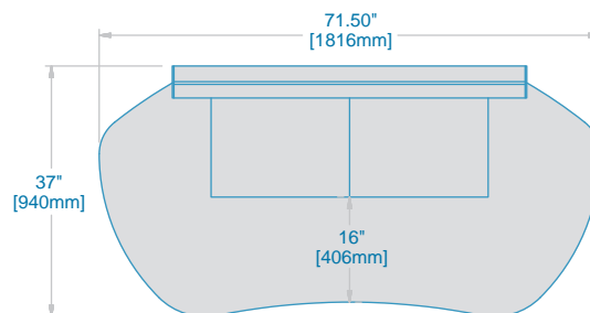
SCALLOPED C-TOP EDGE DETAIL FC-GCX-W2-A
