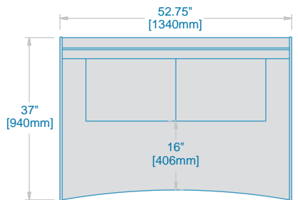
SCALLOPED C-TOP EDGE DETAIL FC-GCX-S2-E
