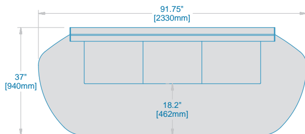
LINEAR C-TOP EDGE DETAIL FC-GCX-S3-B
