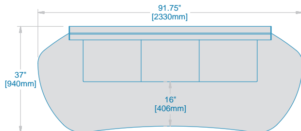
SCALLOPED C-TOP EDGE DETAIL FC-GCX-S3-A
