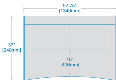
SCALLOPED C-TOP EDGE DETAIL FC-GCX-W2-E
