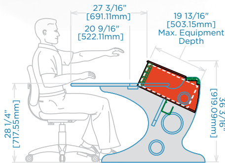
(3) 5RU above countertop rack equipment bays
