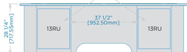
(2) 13RU Fixed 1-Bay Rack equipment cabinets (26RU Total)
