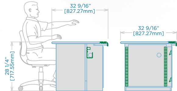
(2) 13RU Fixed 1-Bay Rack equipment cabinets (26RU Total)
