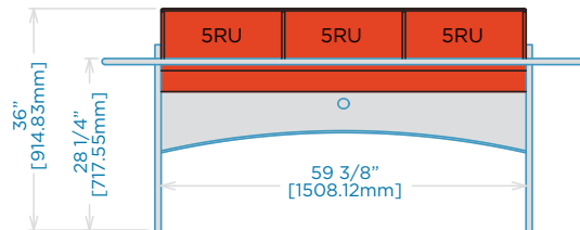
(3) 5RU above countertop rack equipment bays
