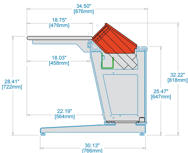
3RU TURRET
